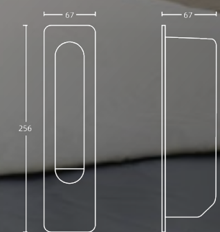
Cutout size (iL-R11) : W64 x H224 mm
